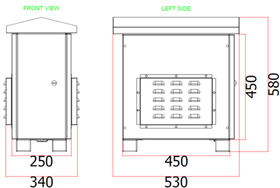
Optional IP54 version (up to 15kVA)
