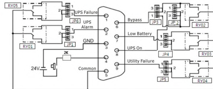
Fig. 3 Connection for ACTIVE OPEN
